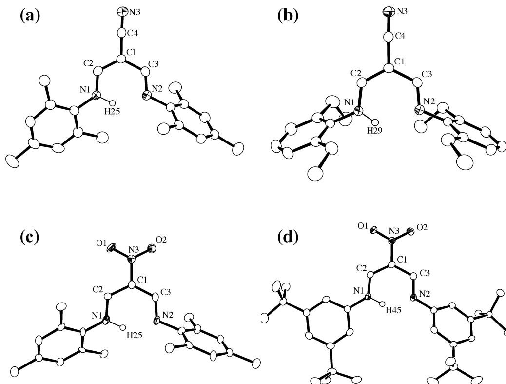
Figure 1. ORTEP drawings of (a) \text{CN}^{\text{L}}\text{MesH} (molecule 1), (b) \text{CN}^{\text{L}}\text{DepH} , (c) \text{NO}_2\text{L}^{\text{MesH}} , and (d) \text{NO}_2\text{L}^{\text{DtbpH}} with 50% probability thermal ellipsoids. Hydrogen atoms except the one at the amino group [H(25) of a, H(29) of b, H(25) of c, and H(45) of d] are omitted for clarity.
